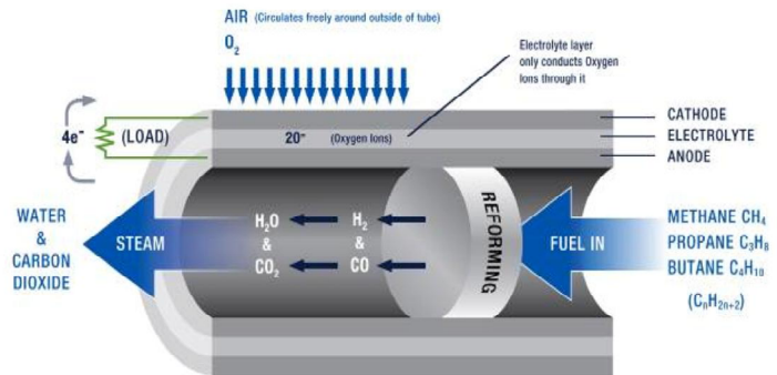
Figure 11. The Atrex Energy SOFC tubular design, and operating principle
