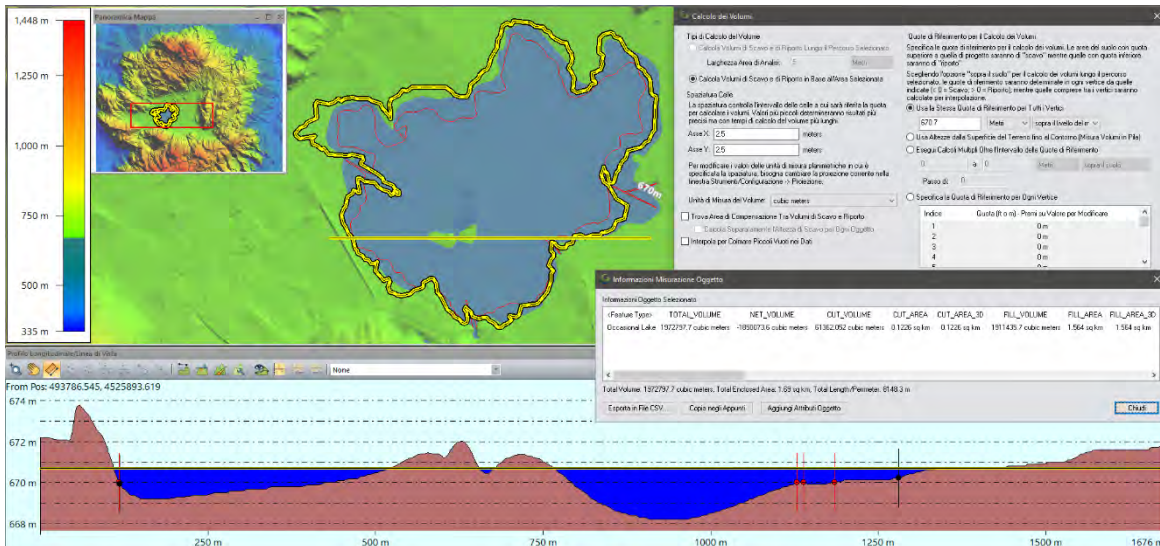
Fig. 6 Volume calculations based on Global Mapper “Calculate Cut-and-Fill Volume” commands with a base height value of 670.7 m above sea level and longitudinal profile along the bottom of the plain with the “Path Profile” tool
