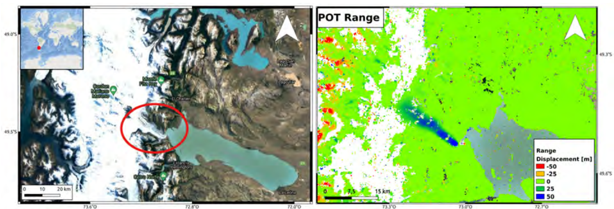
Fig. 1. Viedma glacier (left) and POT range displacement (right) from Sentinel-1 data.
