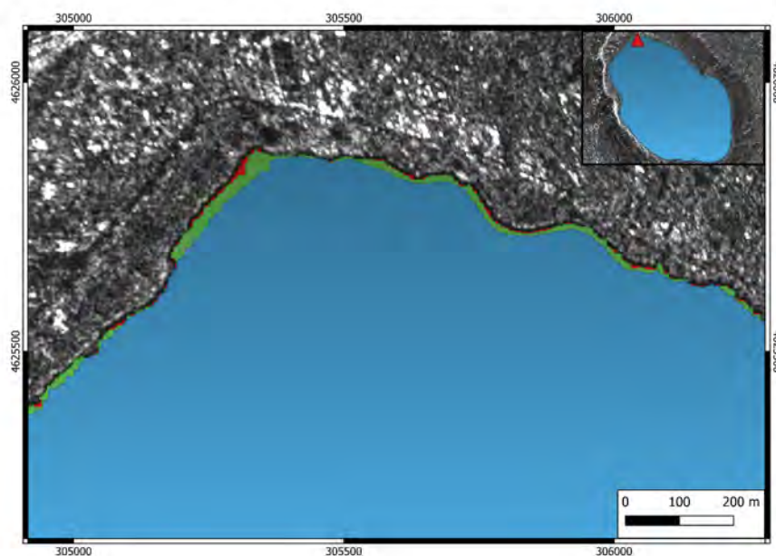
Figure 2: Comparison between the masks of 2017 (red), 2020 (green), and 2023 (blue) of Albano Lake in the northern shoreline (EPSG 32633).
