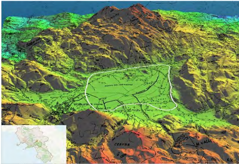
Fig.2 The Dragone plain 3D view: the study area is a depression with a nearly horizontal bottom within Sabato and Calore rivers valleys at an average elevation of 680 m above sea level and an extension of 686 hectares (SIC IT8040014, white contour) and whose centroid is located at Latitude 40° 53' 25.9218" N and Longitude 14° 56' 47.1305" E - WGS84 (Digital elevation model with 5 m resolution and other geographic dataset from Campania Geoportale website and GeneGIS GI, https://parcoregionalemontipicentini.it )
