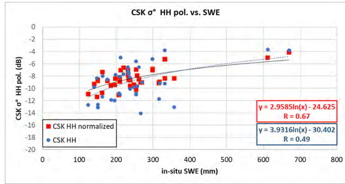
Figure 1. Direct comparison of CSK \sigma^\circ (X-band, HH pol.) and in-situ SWE. Red points correspond to CSK data with LIA normalization, blue correspond to CSK data without LIA normalization.
