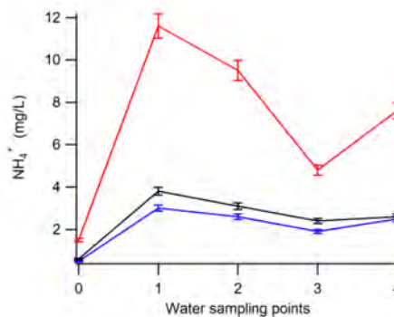
Figure 2 - Ammonium ion ( \text{NH}_4^+ ) concentration (mg/L) measured on water samples collected from Selva del Lamone reserve. Blue line, black line and red line refer to 14 July 2023, 31 July 2023 and 28 August 2023 water sampling campaigns, respectively. Surface water sampling points on X-axis: 0 (Mezzano lake), 1 (Valle Latera), 2 (S. Maria di Sala bridge), 3 (Salabrone waterfalls), 4 (Farnese water treatment plant). %RSD \leq 5%.
