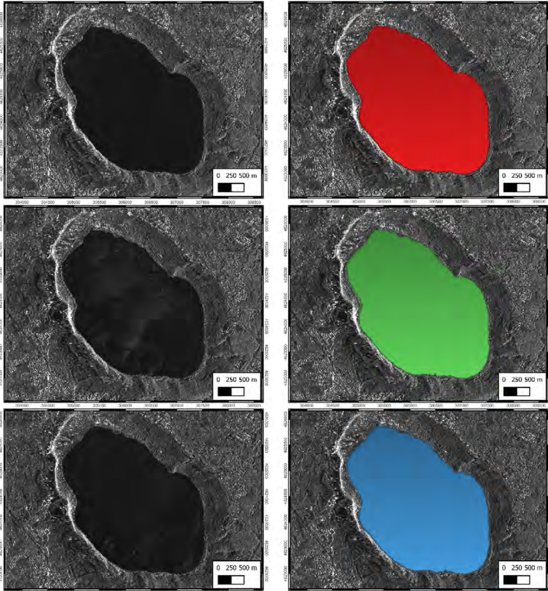
Figure 1: (Left) COSMO-SkyMed-1 image. (Right) COSMO-SkyMed image with lake mask overlay (July 2017 (red) - 2020 (green) - 2023 (blue) – EPSG 32633).
