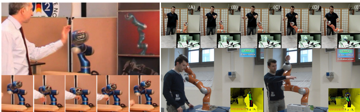
Fig. 69 - (Left) Sensor-less collision detection and robot automatic safe reaction (PHRIENDS), (right) Collision avoidance using a depth sensor, safe coexistence, and human-robot physical collaboration (SAPHARI)
