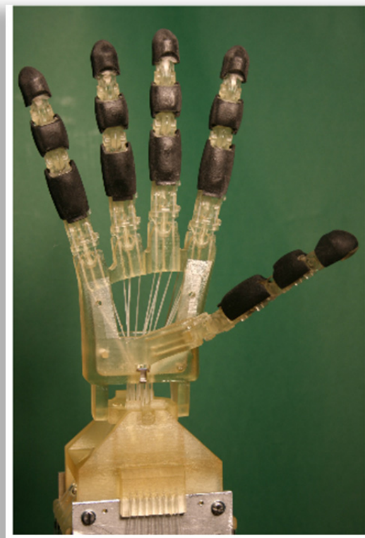
Fig. 32 - Human hand developed in the DEXMART project
