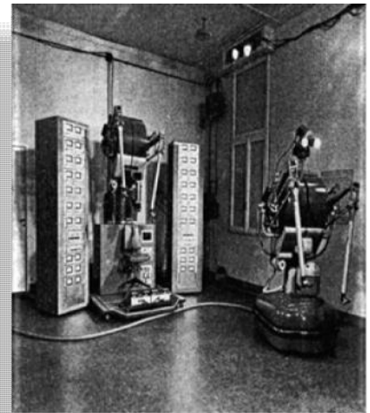
Fig. 54 - Mascot telemanipulator
