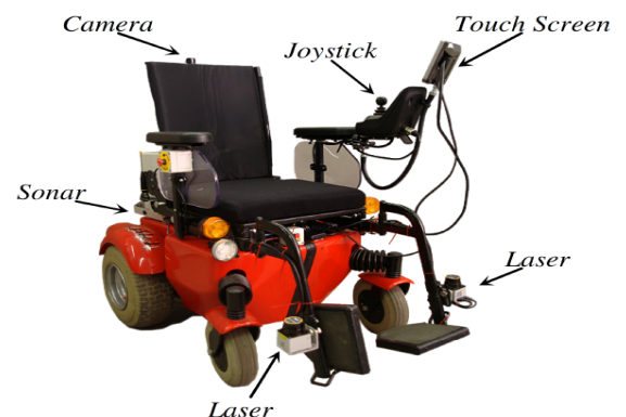
Fig. 20 - Wheelchair realised within LURCH
