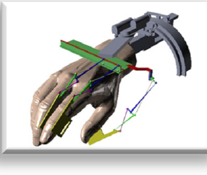
Fig. 31 - Hand active orthosis for the rehabilitation of motor functions at the GRAP
