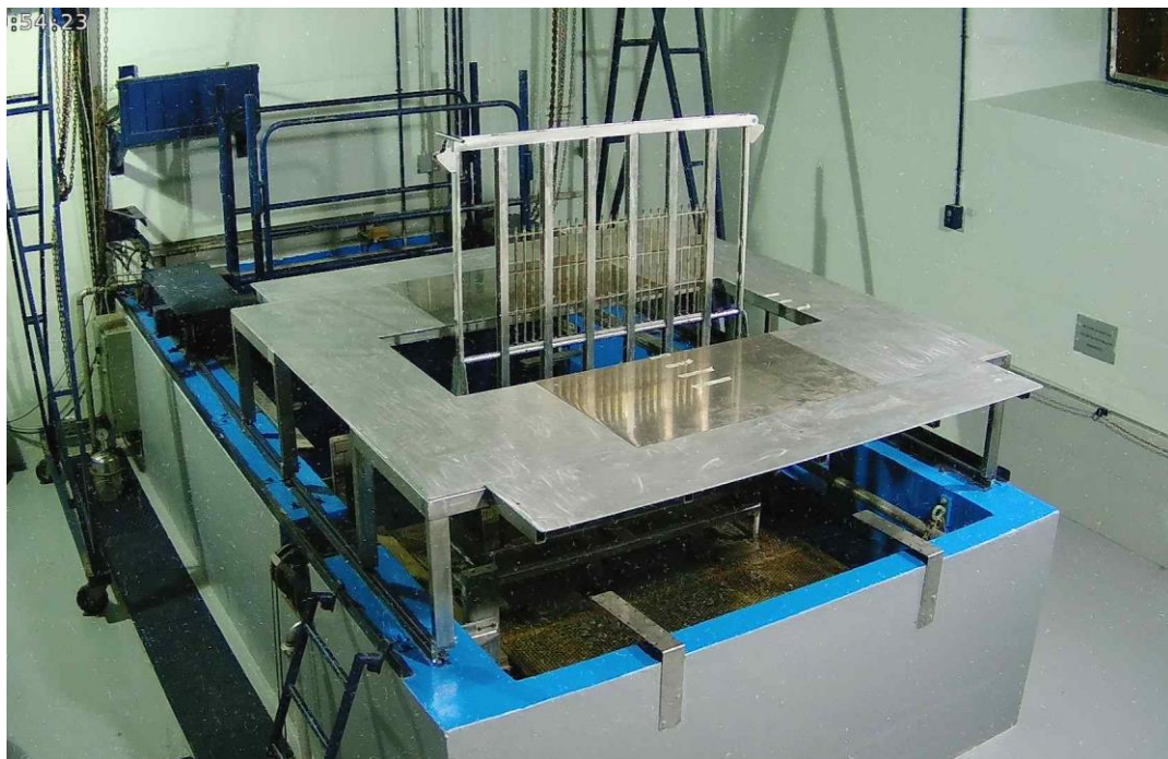
Figure 4 - Irradiation cell with 60 Co sources rack and the platform for sample positioning (picture acquired by local remote camera acquisition).
