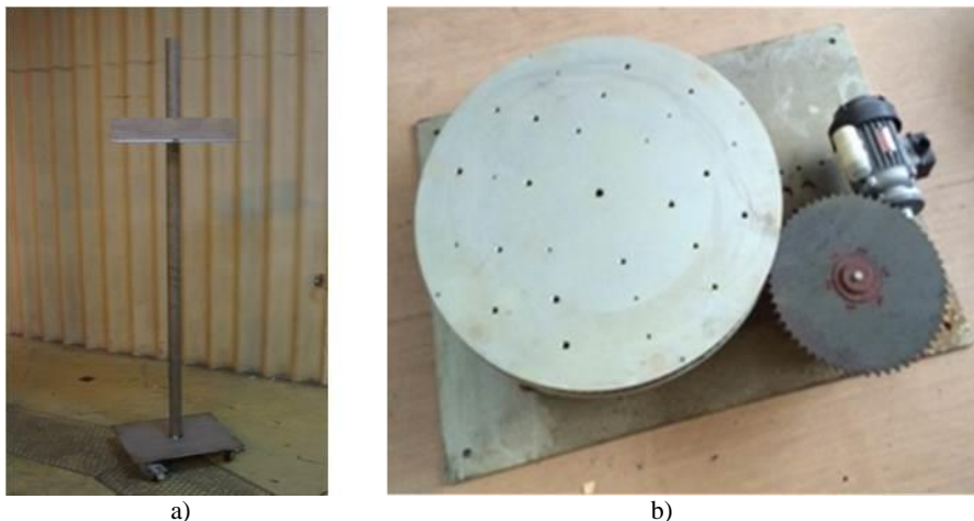
Figure 6 - a) Steel movable mountings; b) rotating platform for uniform irradiation.
